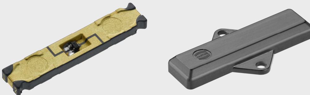
Abbildung 1: Passiver UHF Transponder PT 86 (HT)
